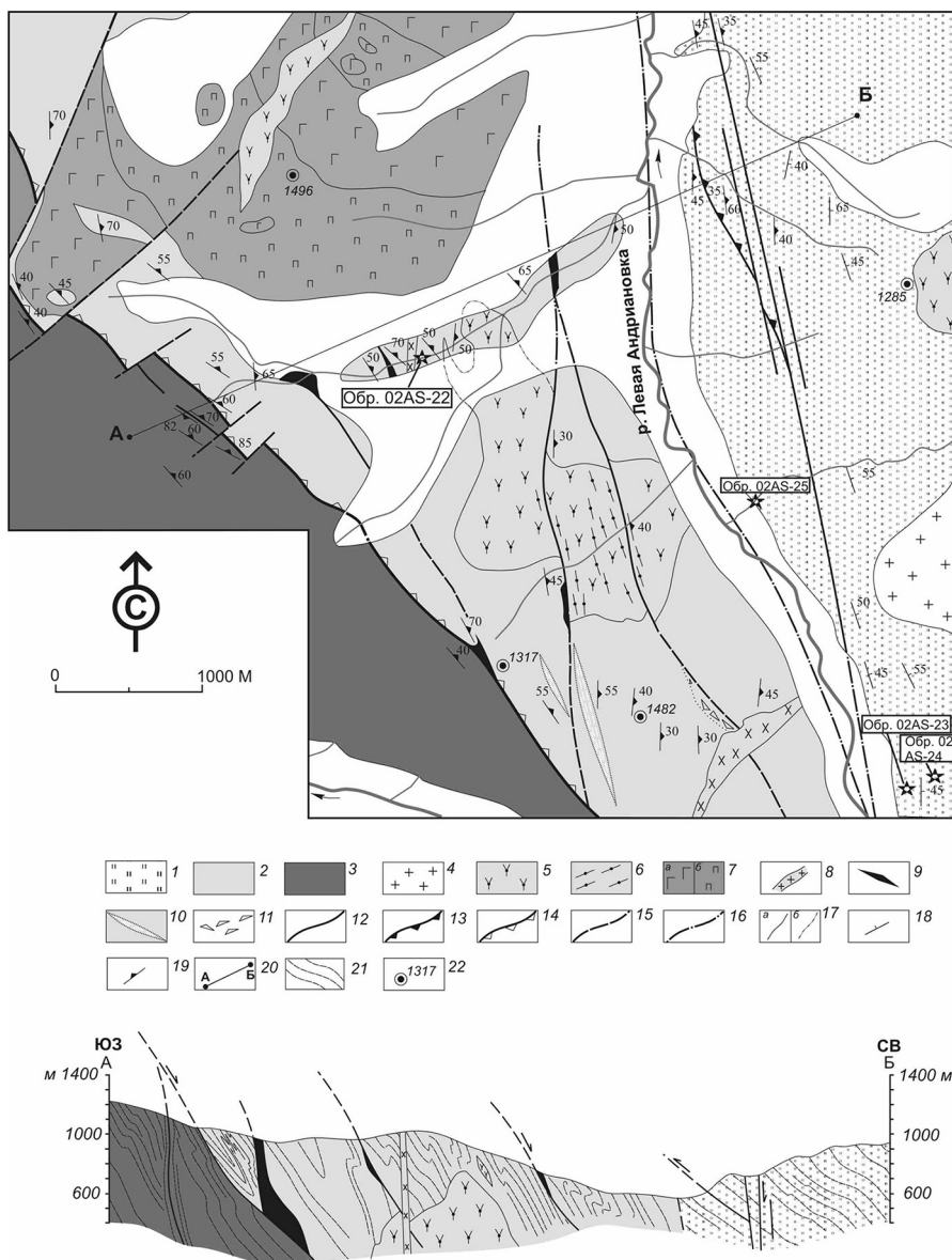
Figure. Geological map of the site in the upper reaches of the Levaya Andrianovka River (Sredinny Ridge, Kamchatka) (according to Ref. [4] using data by M.N. Shapiro): 1–2 – allochthon: 1 – siliceous-volcanogenic deposits of the Irunev Formation, Coniacian – Santonian; 2 – green shales and amphibolites of the Andrianovska Formation, Coniacian – Santonian; 3 – autochthon: biotite-garnet schists of the Kamchatka Series; 4–10 – intrusive formations: 4 – post-collision Miocene granites; 5, 6 – Late Cretaceous syenites (5), including mylonitized ones (6); 7 – complex intrusions of mafic-ultramafic composition, including gabbro (a), gabbro-pyroxenites (b); (8) dikes of granites and diorites; 9 – pyroxenites; 10 – silicification zones; 11 – tectonic (?) breccias; 12–16 – faults (12), including thrusts (12), normal faults (14), supposed faults (15) and hidden under the cover of the Quaternary deposits (16); 17 – geological boundaries (a), including those assumed under the cover of Quaternary deposits (b); 18–19 – occurrence elements: 18 – bedding, 19 – schistosity; 20 – cut line; 21 – layering (schistosity) on the profile; 22 – absolute elevations.
